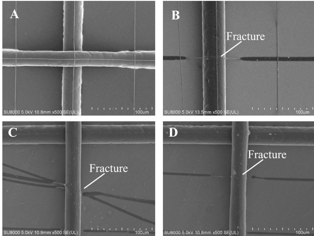
Figure S2. PCL/nHA fibers with nHA concentrations of 0.5% (A), 1% (B), 2% (C), 4% (D) when deposited on previously printed microscale fibers.
