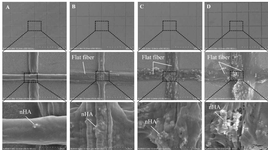
Figure S1. PCL/nHA fibers with nHA concentrations of 0.5% (A), 1% (B), 2% (C), 4% (D).
