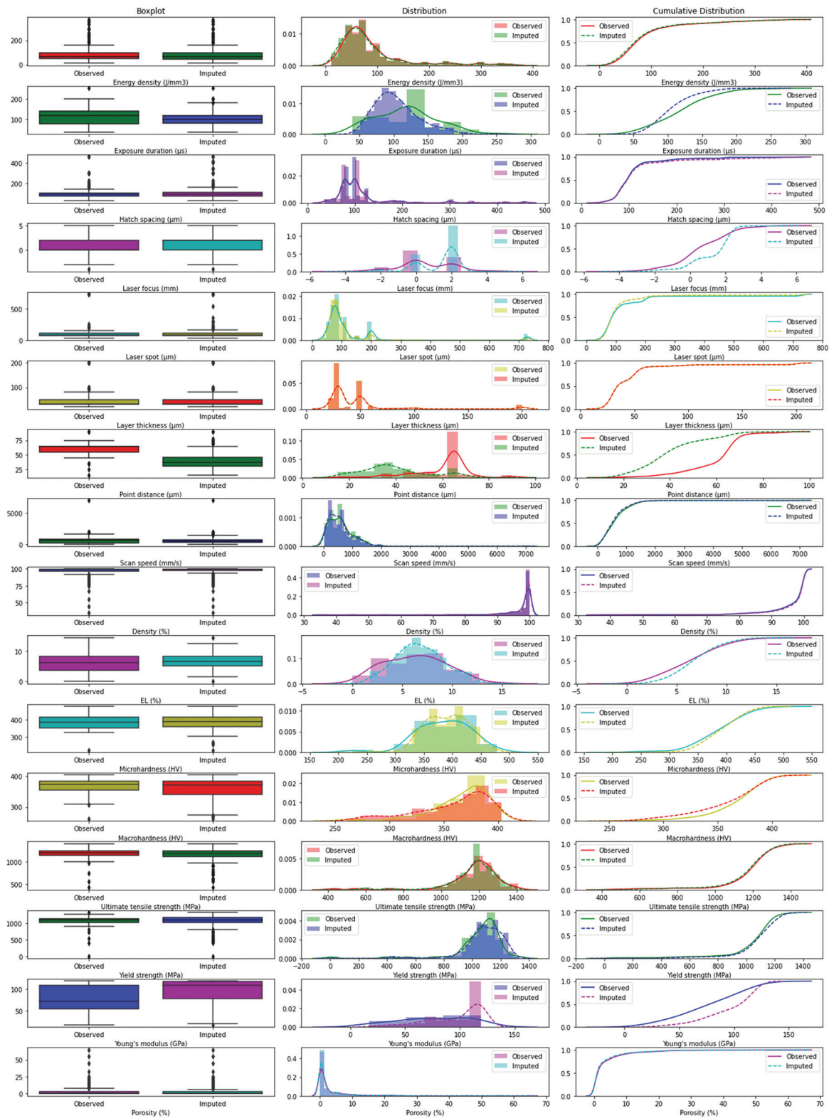
Figure S3. Graph imputation neural network Imputation data distribution.
