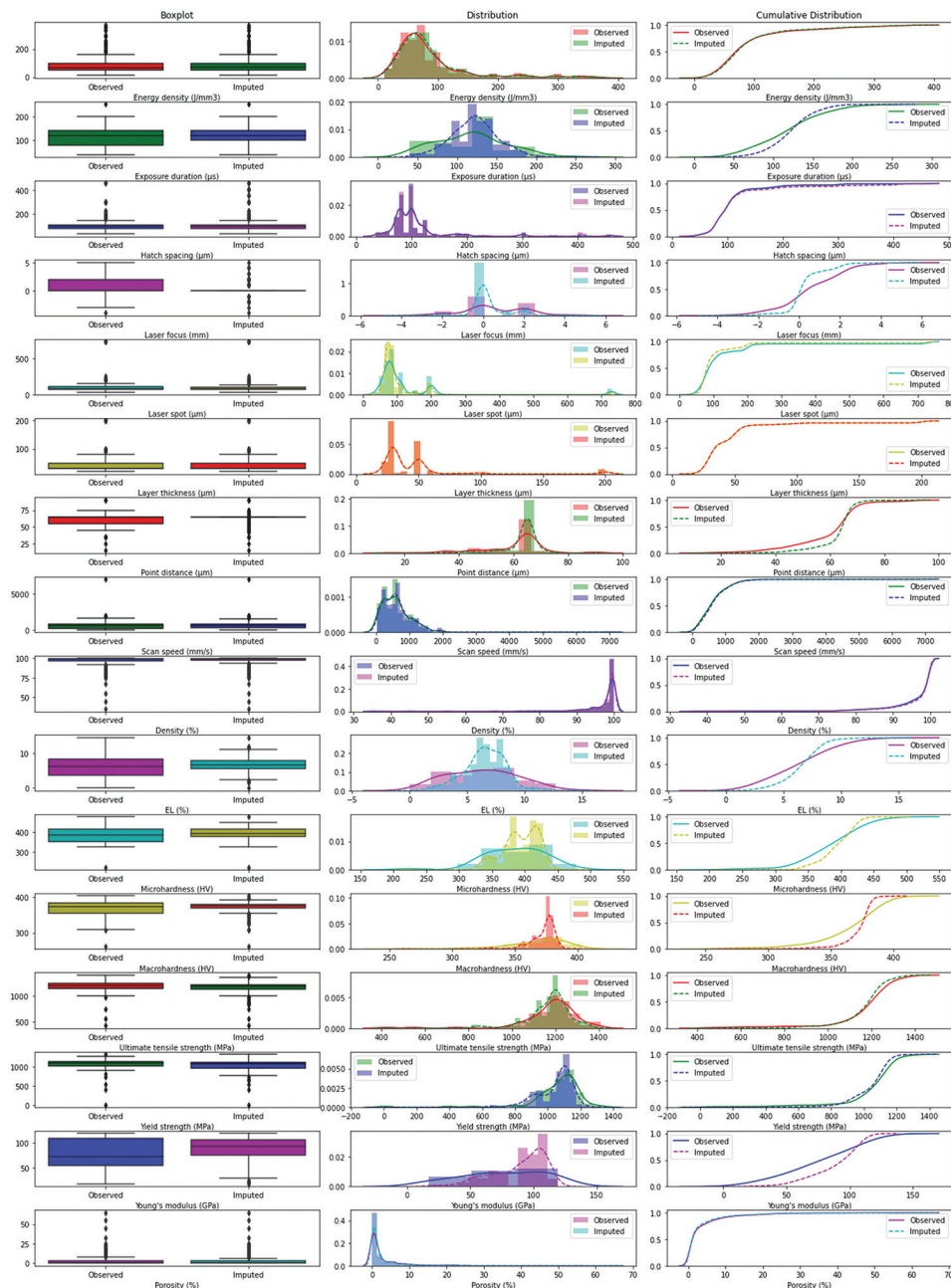
Figure S1. k-nearest neighbor imputation data distribution.
