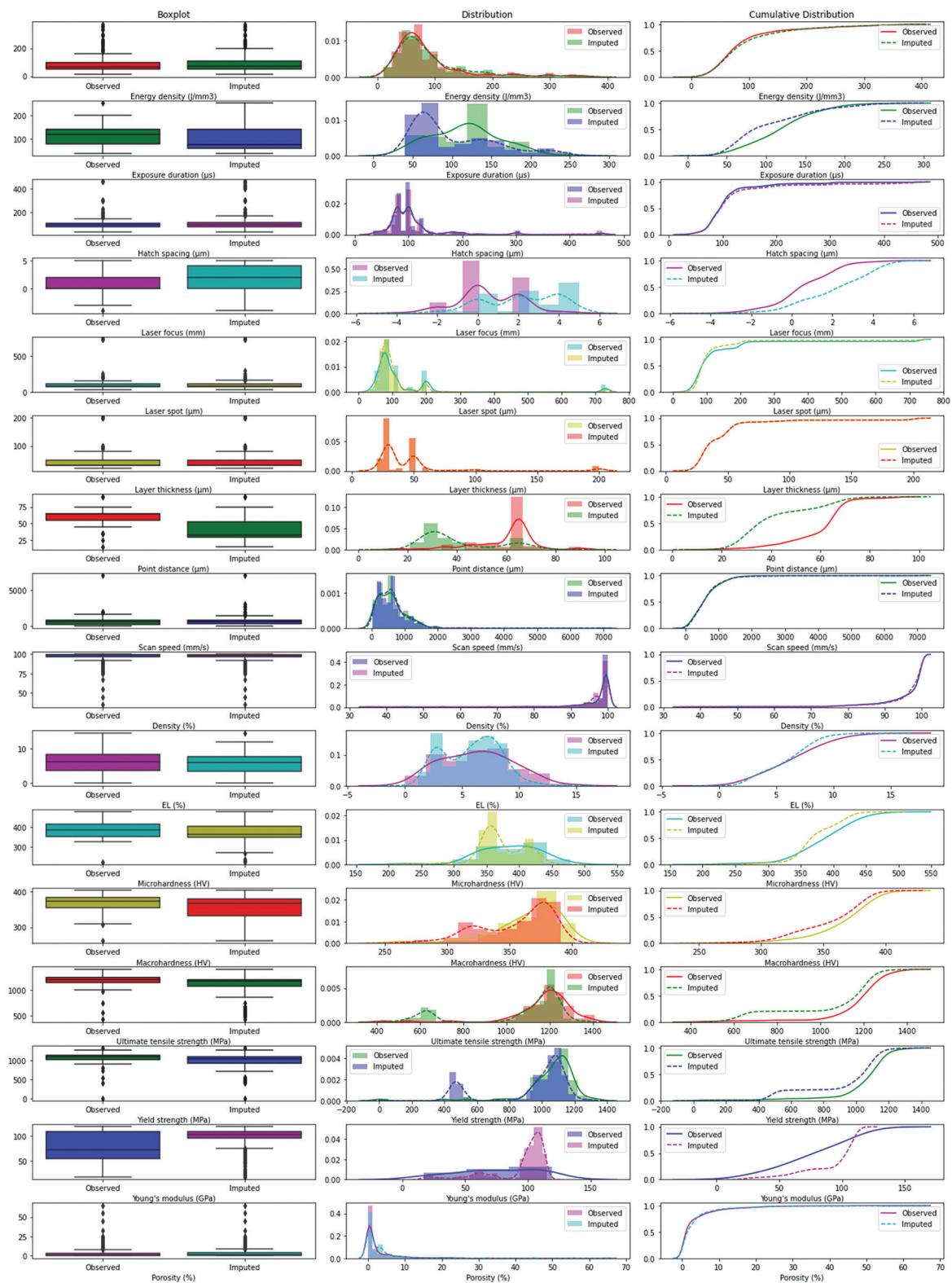
Figure S2. Multivariate imputation by chained equations imputation data distribution.
