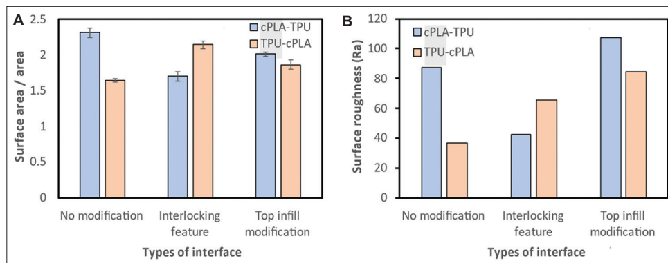
Figure S1. Graphs showing the (A) surface area/area ratio and (B) surface roughness ( R_a ) for the last printed interfaces.
