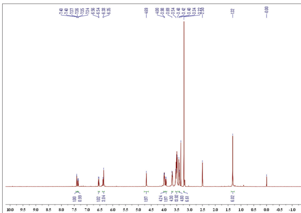
Figure S1. 1 H NMR (400 MHz, DMSO- d 6 ) spectrum of Compound 4.
