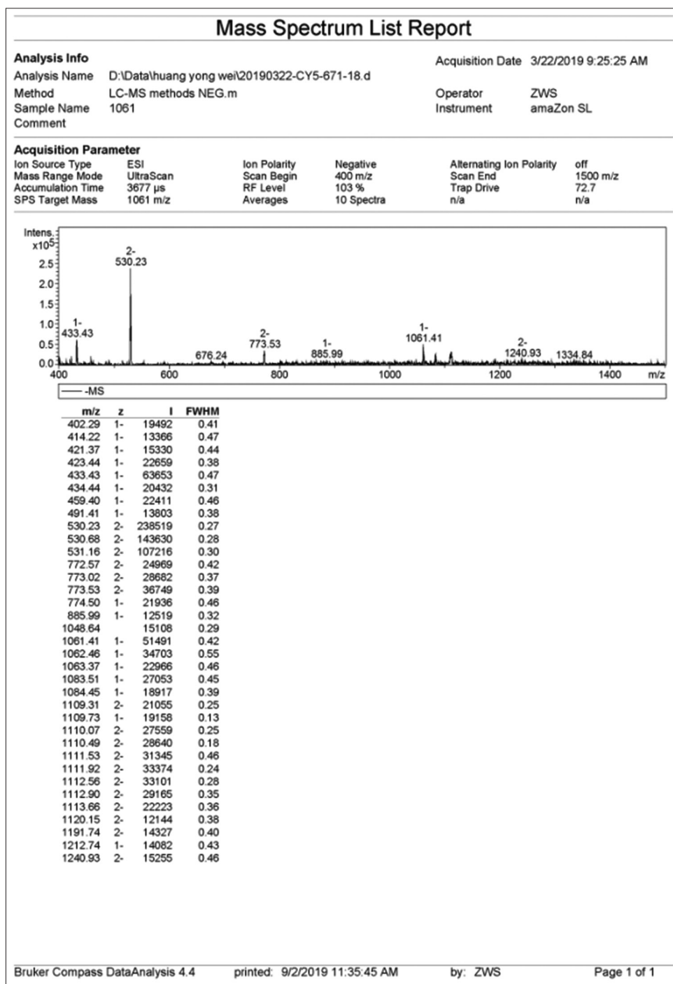
Figure S4. MS (ESI) spectrum of Cy5-664.
