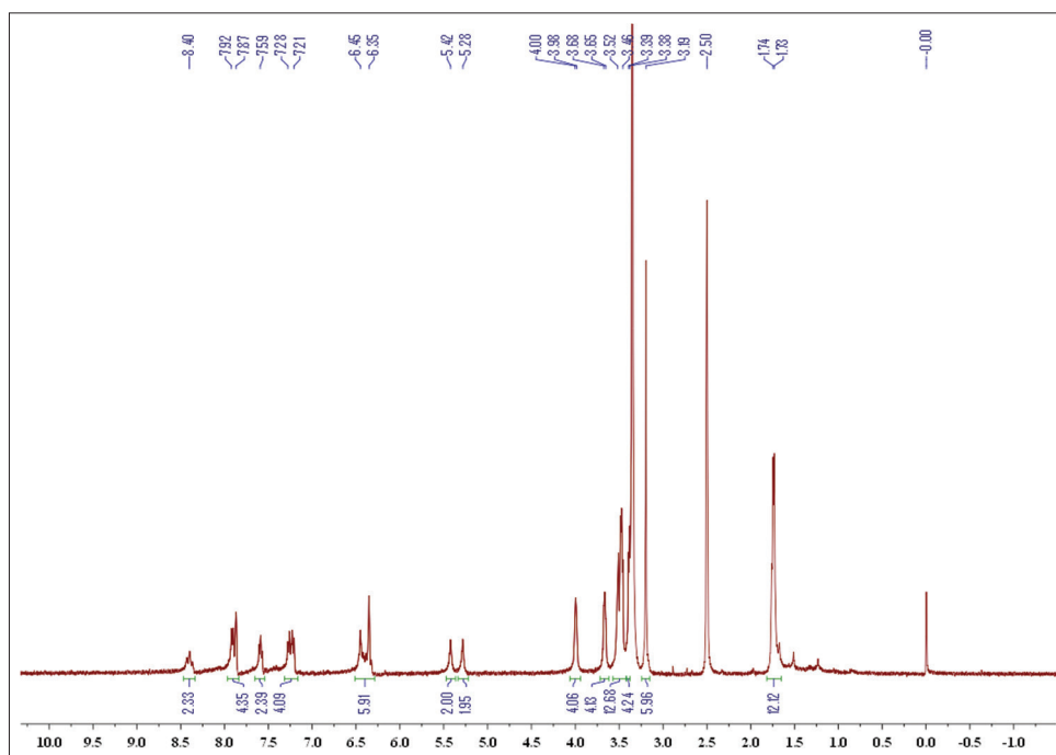
Figure S2. ^1\text{H} NMR (400 MHz, \text{DMSO}-d_6 ) spectrum of Cy5-664.
