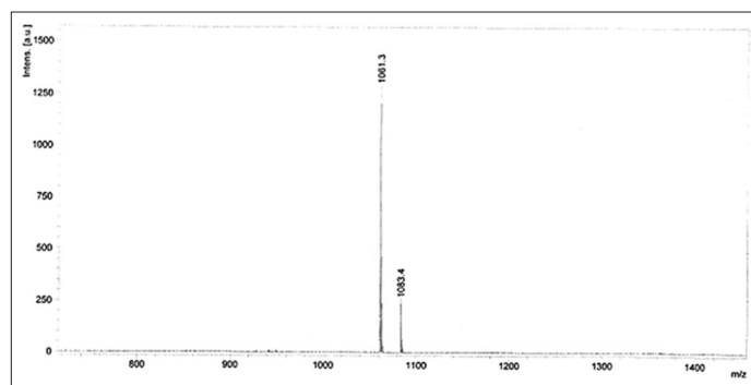
Figure S3. HRMS (ESI) spectrum of Cy5-664.
